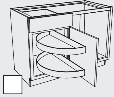
Blind Corner with Revolving Shelf Block 3155
