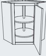
Diagonal Wall with Lazy Susan Block 1520
