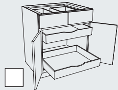
Base with Roll Out Trays Block 4010
