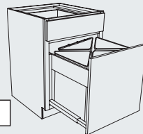
Recycle Base Block 4130
