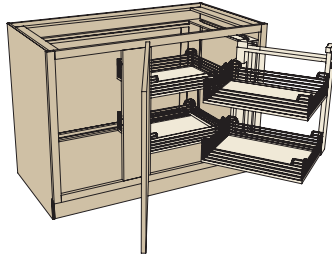
1 Blind Corner with Magic Corner Shelves Block 3159
