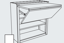
Wall Cabinet with Bifold Door Block 1120
