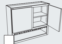
Wall with Stem Glass Rack Block 2140
